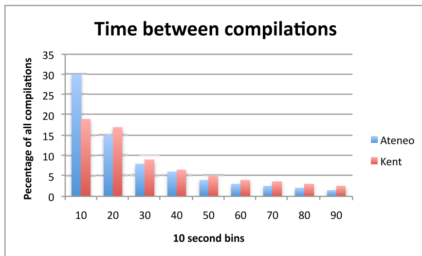
Figure 2: The time between successive compilations as observed in students at the University of Kent and the Ateneo de Manila. (Full corpus, both institutions.)
