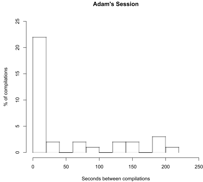
Figure 3: Distribution of time spent between compilations in Adam's session.
