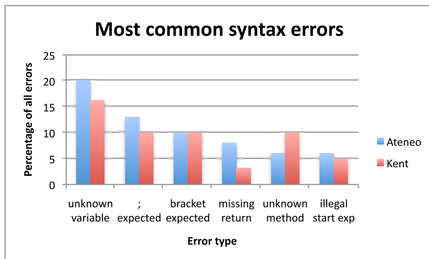
Figure 1: The most common syntax errors encountered by students at the University of Kent and the Ateneo de Manila. (Full corpus, both institutions.)
